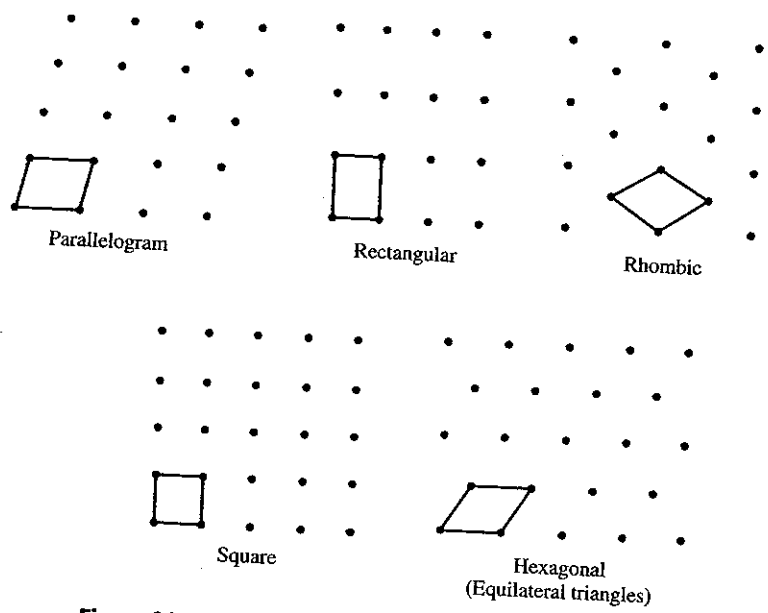
Figure 28.20 Possible lattices for plane periodic patterns
